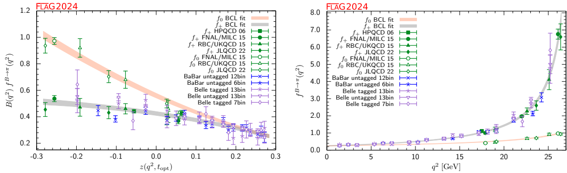
Figure 31: Lattice and experimental data for f_{+}^{B \rightarrow \pi}(q^2) and f_0^{B \rightarrow \pi}(q^2) versus z (left panel) and q^2 (right panel). Experimental data has been rescaled by the value for |V_{ub}| found from the joint fit. Green symbols denote lattice-QCD points included in the fit, while blue and indigo points show experimental data divided by the value of |V_{ub}| obtained from the fit. The grey and orange bands display the preferred N^+ = N^0 = 3 BCL fit (five z -parameters and |V_{ub}| ).
